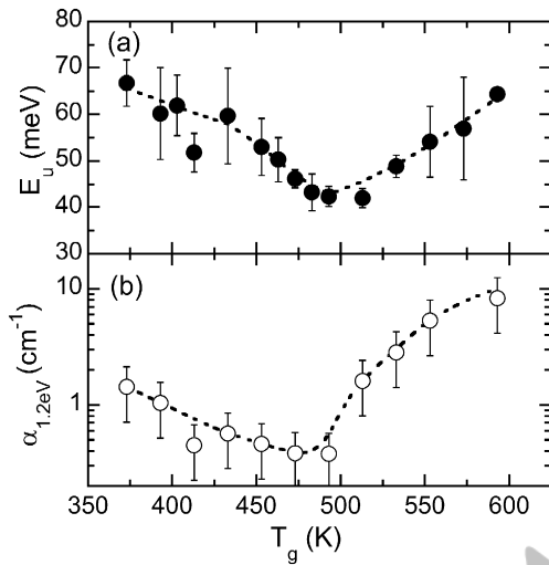
Fig. 7. (a) Urbach energy, E_U , and (b) absorption coefficient at 1.2 eV, \alpha_{1.2\text{eV}} , as a function of T_g . E_U is ranged from \approx 40 meV to \approx 65 meV, and minimized around T_g = 493 K. (b) \alpha_{1.2\text{eV}} is ranged from \approx 0.3 \text{cm}^{-1} to \approx 10 \text{cm}^{-1} for a-Si:H films grown at T_g = 373 K to 593 K. The dotted lines are guides to the eyes.
