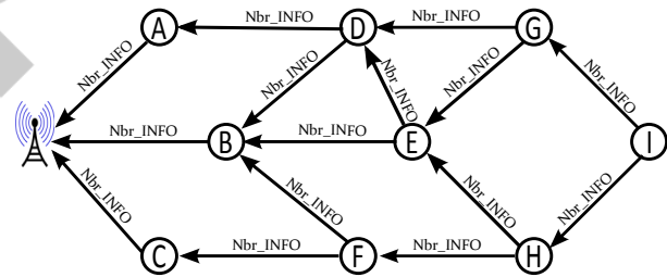
Figure 1: Nodes send the Nbr\_INFO packet to the base station.
