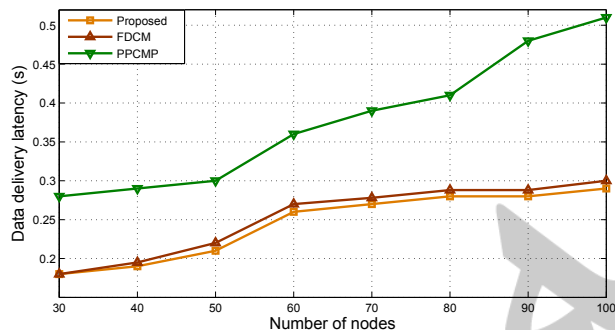
Figure 5: End to End Latency
