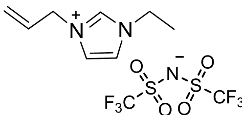
Scheme 1. Structure of Polymerizable RTIL, [AllylEtIm][Tf 2 N]
