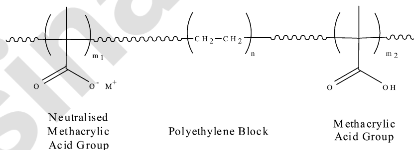
Fig. 9. Structure of a partially neutralized random EMAA ionomers where M^+ can be sodium, potassium, zinc, copper or an iron cation [224].
