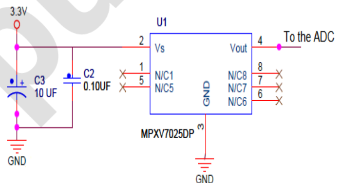
Fig 8: Pressure sensor connections
