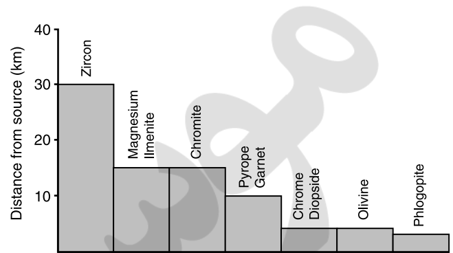
Fig. 5. Relative abundance of indicator minerals at varying distance from source in unglaciated Australian terrains (modified from Atkinson 1989).
