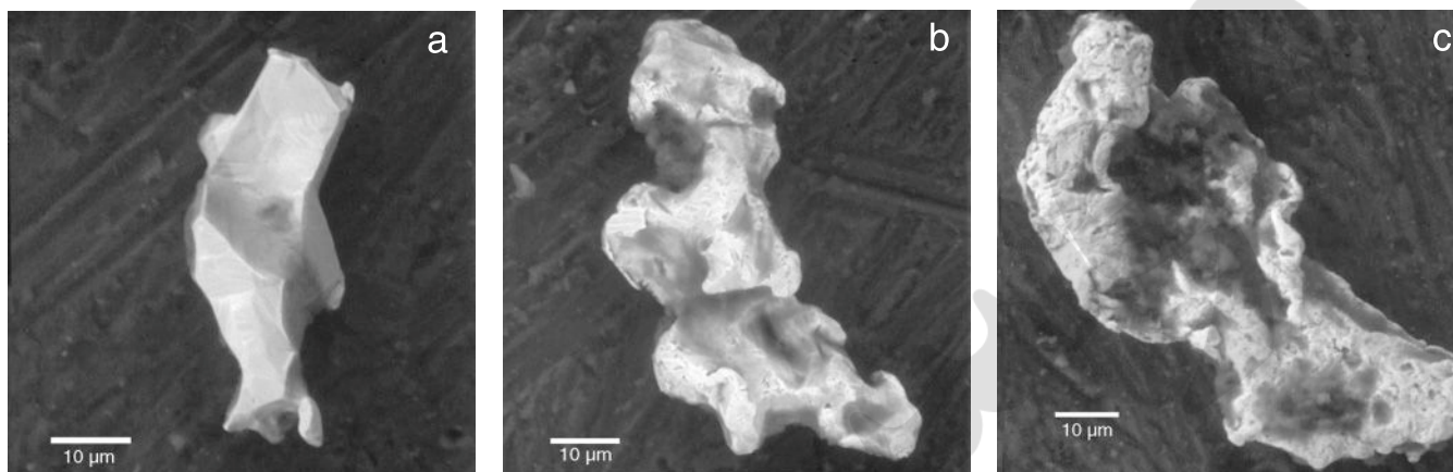
Fig. 1. Secondary electron images of gold grains from till showing the three conditions routinely documented for gold grains: (a) pristine gold grain with equant molds suggestive of former quartz–feldspar–carbonate–sulphide gangue; (b) modified gold grain with vestiges of equant molds and edges that are slightly curled; and (c) reshaped gold grain showing pitted surfaces and well curled edges (from McClenaghan 2001).
