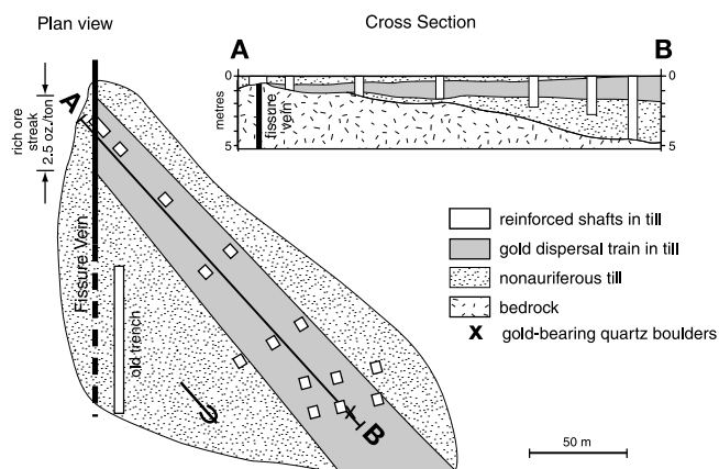
Fig. 2. Location of till samples collected by Prest in 1896 to trace the source of gold-bearing quartz boulders (indicated by x) and define a ribbon-shaped gold grain dispersal train in Nova Scotia, Canada (modified from Stea & Finck 2001).
