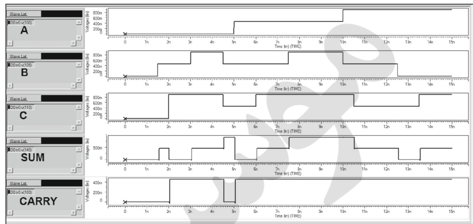
Fig. 17 Transient response of ternary full adder
