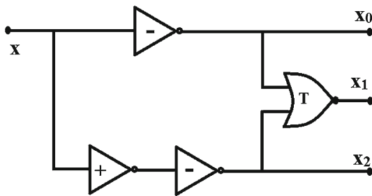
Fig. 5 Ternary decoder circuit
