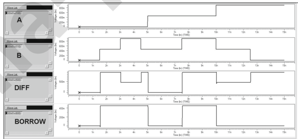
Fig. 19 Transient response of ternary half subtractor
