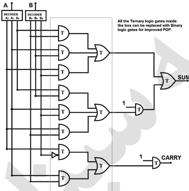
Fig. 6 Structure of ternary half adder
