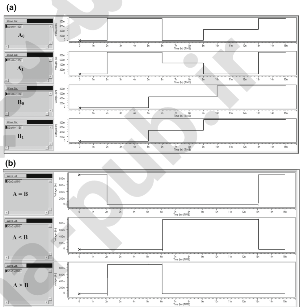
Fig. 21 a Behavior of 2-bit comparator inputs— A_0 , A_1 , B_0 & B_1 . b Behavior of 2-bit comparator outputs— A = B , A < B & A > B
