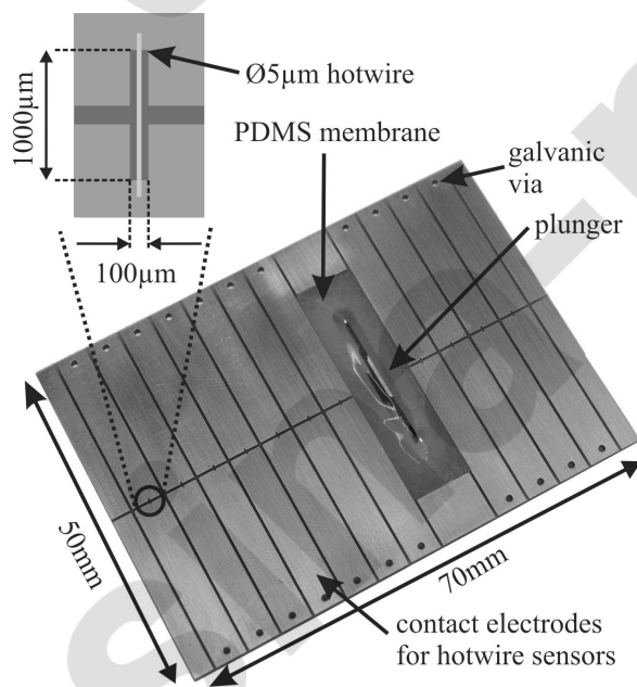
Figure 6) Complete system for active delay of transition with PCB, actuator, membrane, and hot wire flow sensors.
