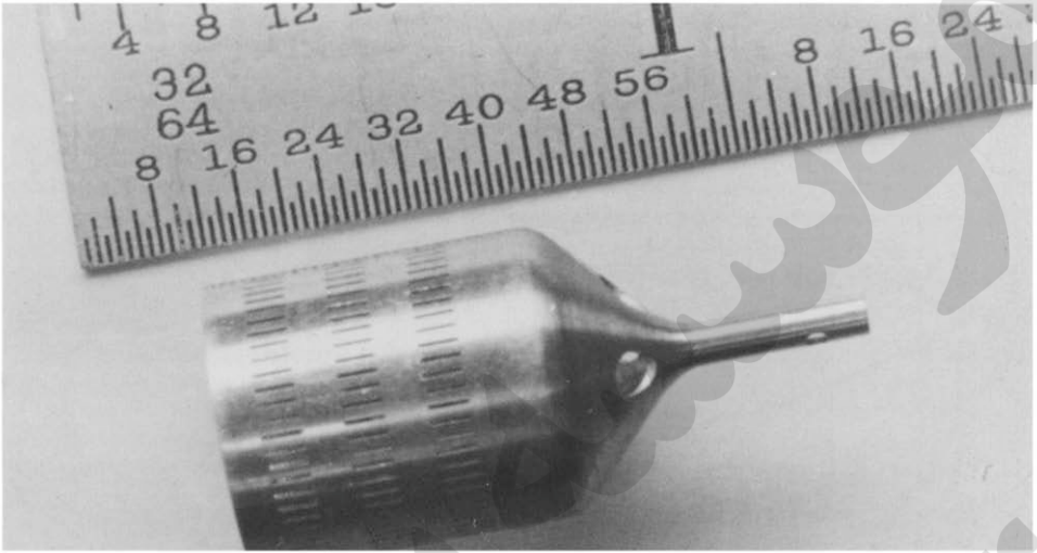
Figure 11 - Variable extrusion pressures permit even fragile components to be reliably processed.
